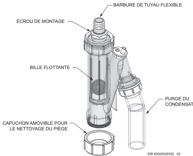
Figure 2-1 Siphon du condensat
